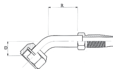
Long pilot "O" ring wartel, 45° - pijp aansluiting "O" ring female swivel, 45° - tube connection "O" ring femelle tournant, 45° - tube connection
