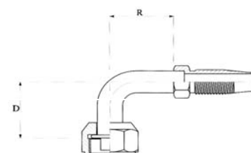
Long pilot "O" ring wartel 90° – pijp aansluiting "O" ring female 90° swivel – tube connection "O" ring femelle tournant 90° – tube connection
