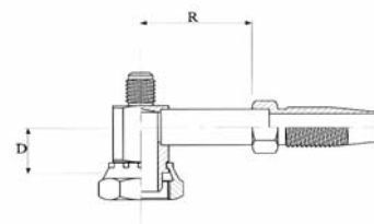
Tube "O" compressor wartel, 90° / R12 ventiel Tube "O" compressor fitting, 90° / R12 valve Raccord tube "O" compresseur, 90° / R12 valve
