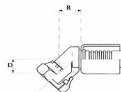
Tube "O" compressor wartel, 45° gebogen Tube "O" compressor fitting, 45° elbow Raccord tube "O" compresseur, coudé 45°
