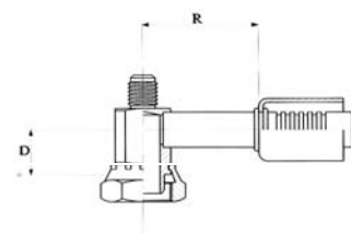
Tube "O" compressor wartel, 90°/R12 ventiel Tube "O" compressor fitting, 90°/R12 valve Raccord tube "O" compresseur, 90°/R12 valve
