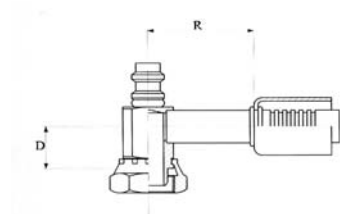
Tube "O" compressor wartel, 90°/R134 ventiel Tube "O" compressor fitting, 90°/R134 valve Raccord tube "O" compresseur, 90°/R134 valve
