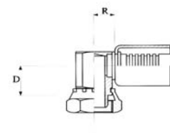
Tube "O" compressor wartel, 90° gebogen Tube "O" compressor fitting, 90° elbow Raccord tube "O" compresseur, coudé 90°
