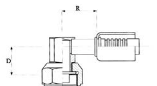
"O" ring wartel pijp, bloktype, 90° "O" ring female swivel, 90°, block type "O" ring femelle tournant, 90°, block
