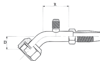
"O" ring wartel, 45°/R12 ventiel "O" ring female swivel, 45°/R12 valve "O" ring écrou tournant, 45°/R12 valve
