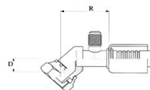
Tube "O" compressor, 45°/R12 ventiel Tube "O" compressor fitting, 45°/R12 valve Raccord tube "O" compresseur, 45°/R12 valve
