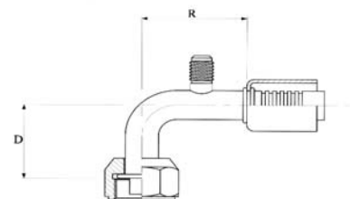
"O" ring wartel, 90°/R12 ventiel "O" ring swivel, 90°/R12 valve "O" ring écrou tournant, 90°/R12 valve
