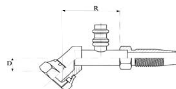
Tube "O" compressor wartel, 45° / R134 ventiel Tube "O" compressor fitting, 45° / R134 valve Raccord tube "O" compresseur, 45° / R134 valve
