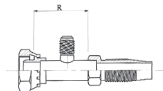
Tube "O" compressor wartel / R12 ventiel Tube "O" compressor fitting / R12 valve Raccord tube "O" compresseur / R12 valve
